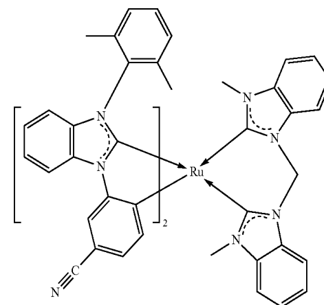
Compound 23
