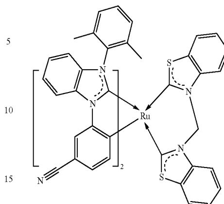
Formula XV
