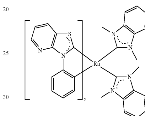
Compound 8
