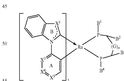
Compound 13
