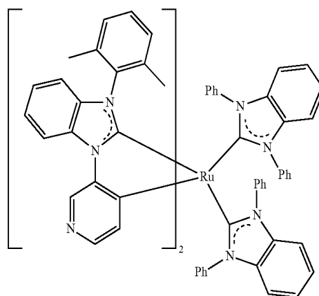
Compound 1
