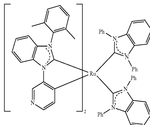
Compound 1
