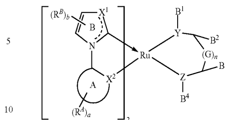
Compound 10
