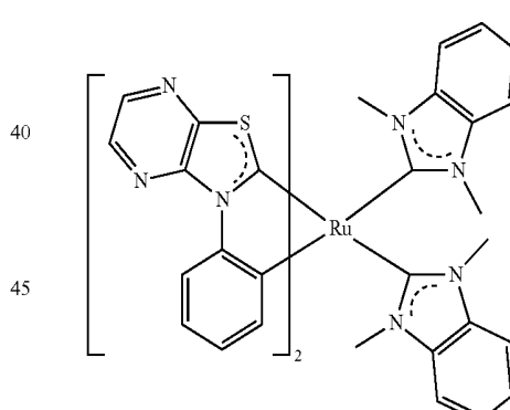
Compound 9
