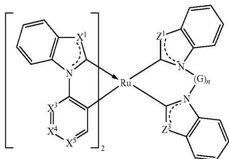
Formula XVI
