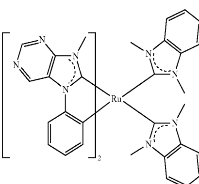
Compound 5
