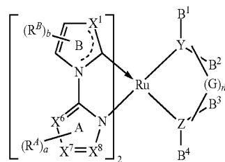
Formula XIV
