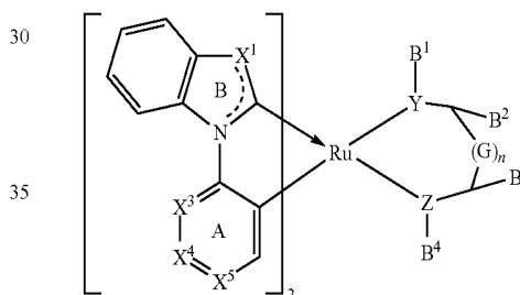
Compound 12
