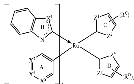
Formula VIII
