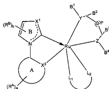
Formula I
