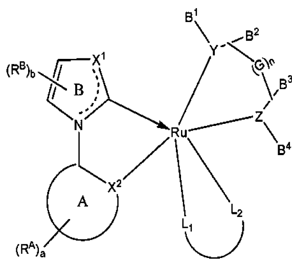
Formula I
