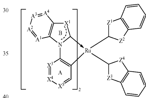
Formula VI
